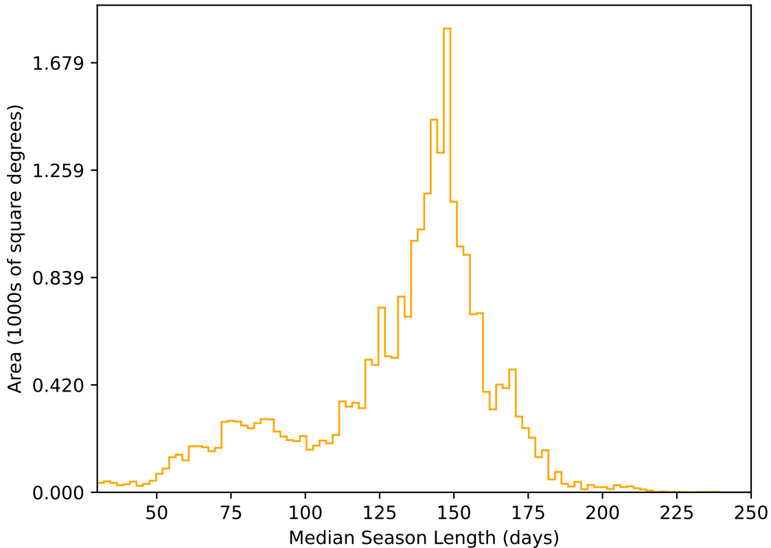
too_elab_r32_d3_giz_v3.4_10yrs All sky r band: Median Season Length
