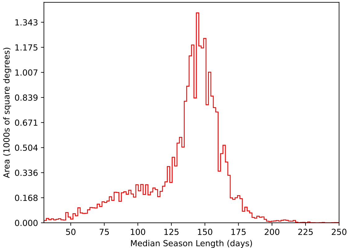
too_elab_r32_d3_giz_v3.4_10yrs All sky i band: Median Season Length
