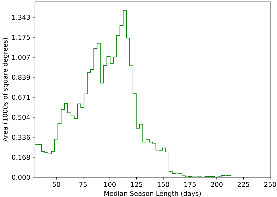
too_elab_r32_d3_giz_v3.4_10yrs All sky g band: Median Season Length
