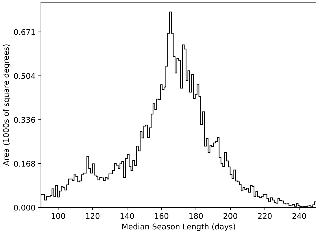
too_elab_r32_d3_giz_v3.4_10yrs All sky all bands: Median Season Length
