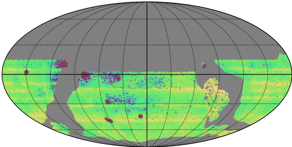
too_elab_r32_d3_giz_v3.4_10yrs WFD: Median Intra-Night Gap
