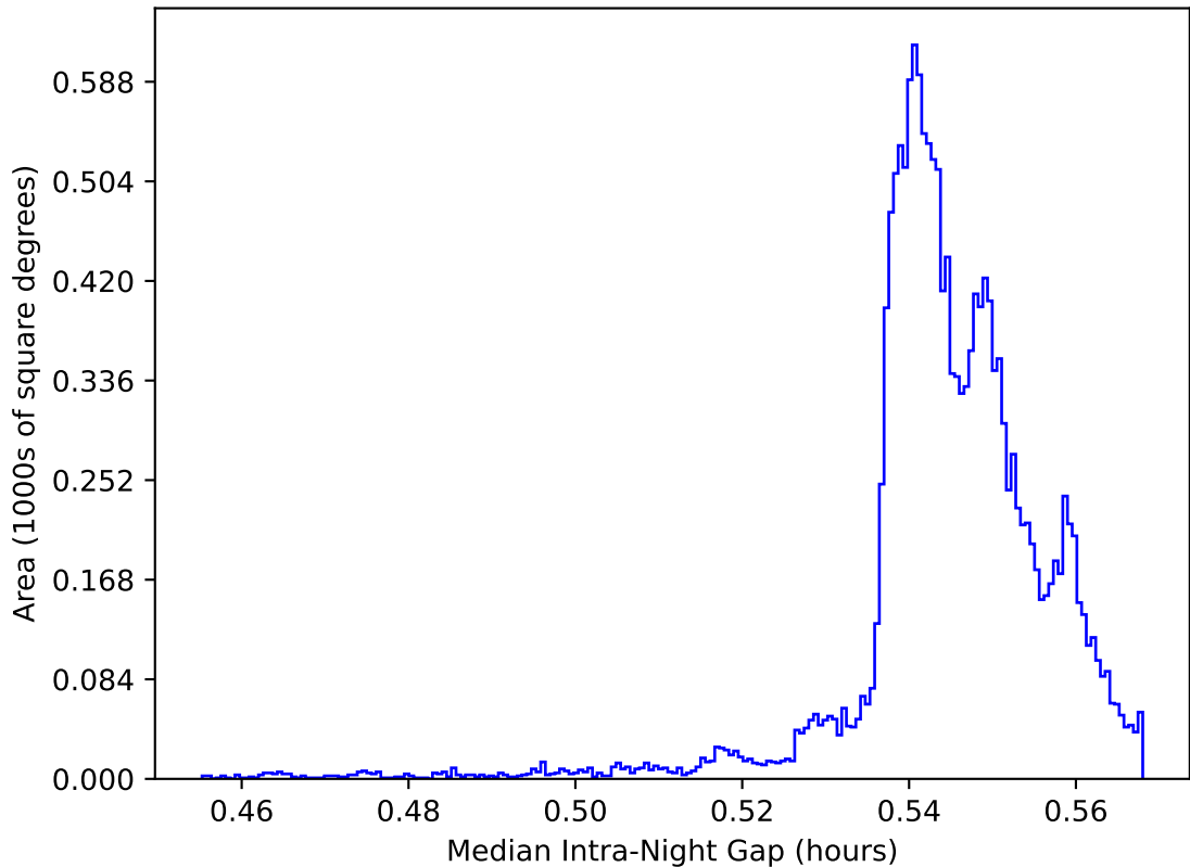
too_elab_r32_d3_giz_v3.4_10yrs WFD: Median Intra-Night Gap
