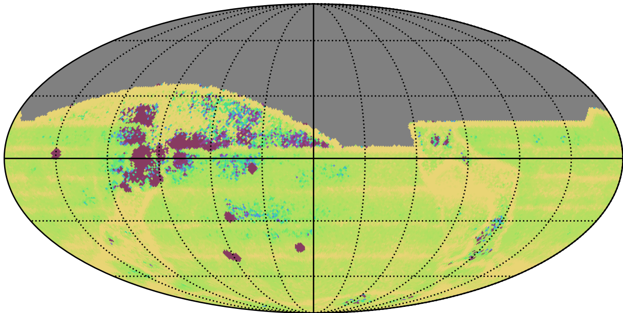
too_elab_r32_d3_giz_v3.4_10yrs All sky: Median Intra-Night Gap
