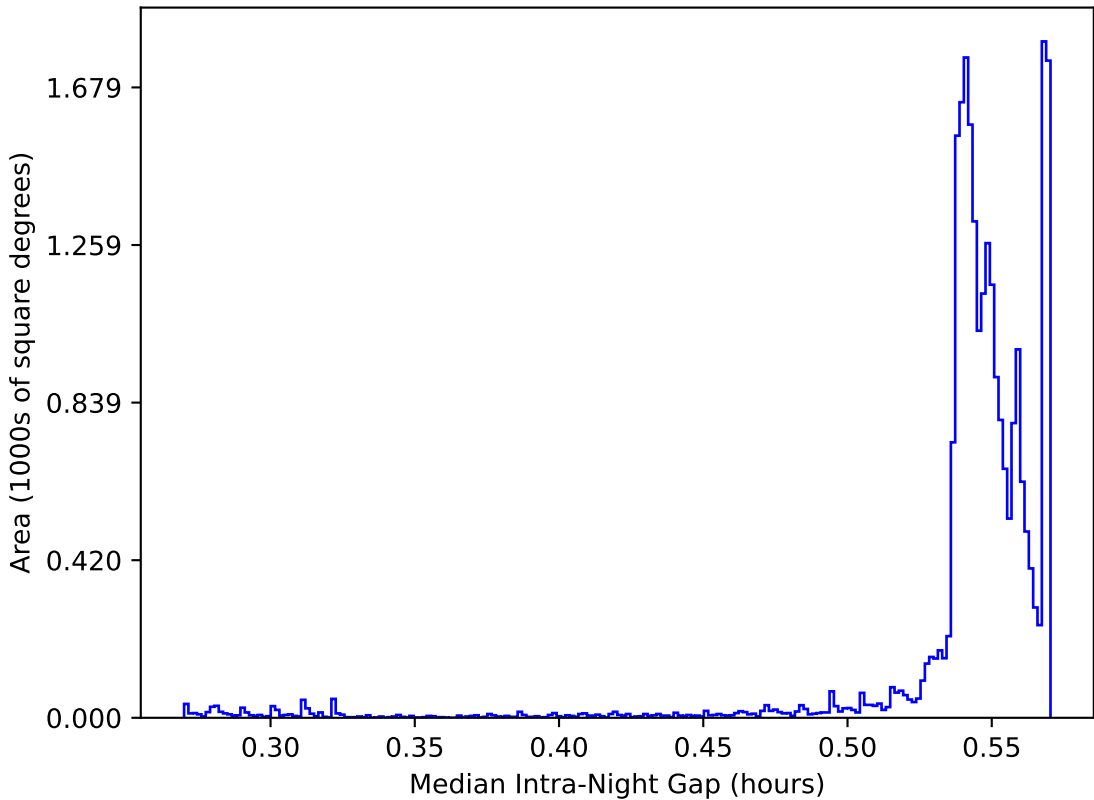
too_elab_r32_d3_giz_v3.4_10yrs All sky: Median Intra-Night Gap
