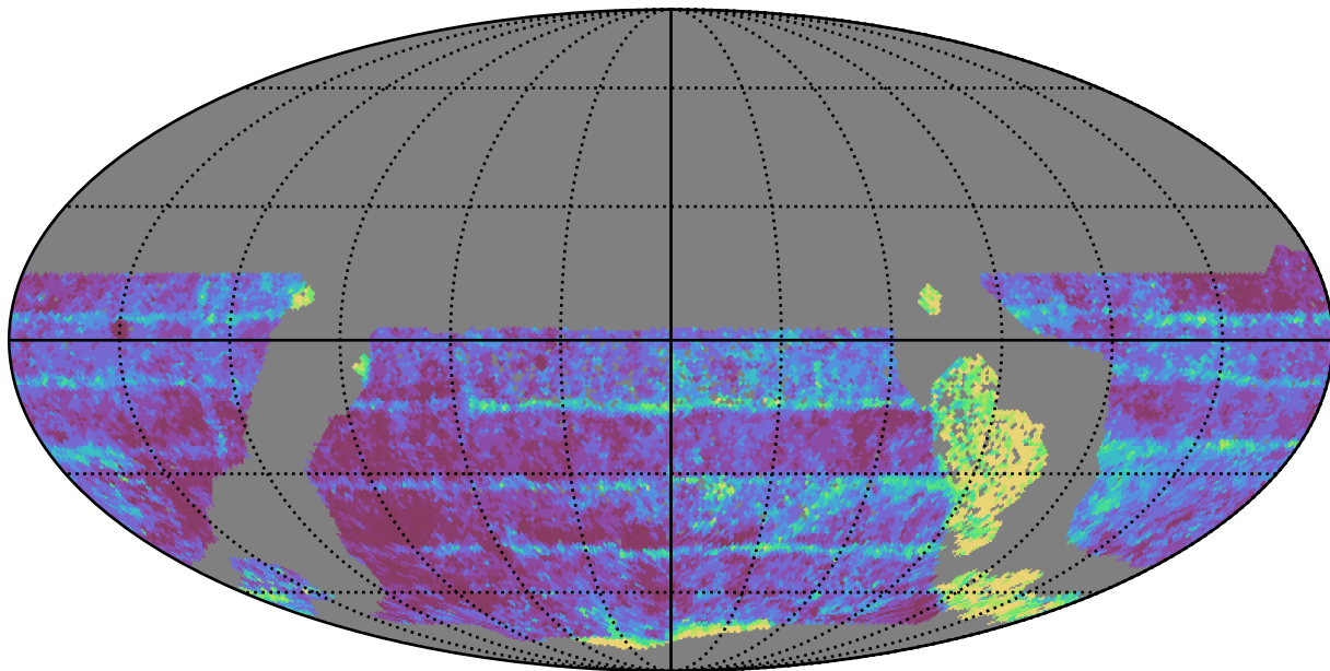
too_elab_r32_d3_giz_v3.4_10yrs WFD z band: Median Inter-Night Gap
