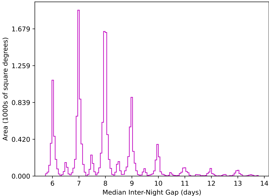
too_elab_r32_d3_giz_v3.4_10yrs WFD z band: Median Inter-Night Gap
