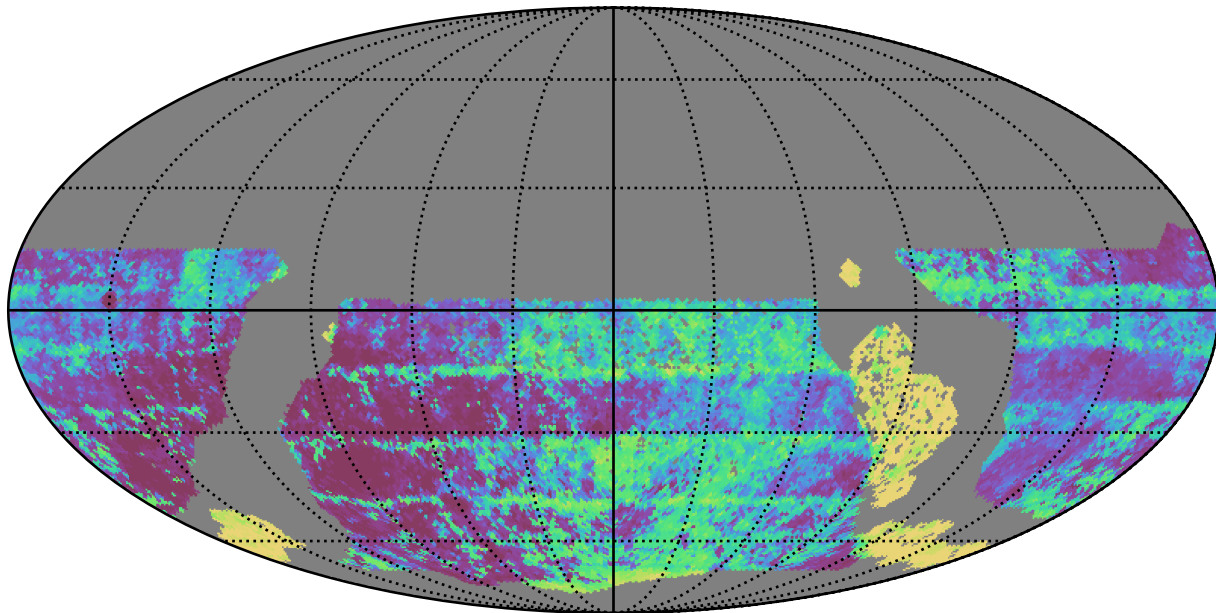
too_elab_r32_d3_giz_v3.4_10yrs WFD y band: Median Inter-Night Gap
