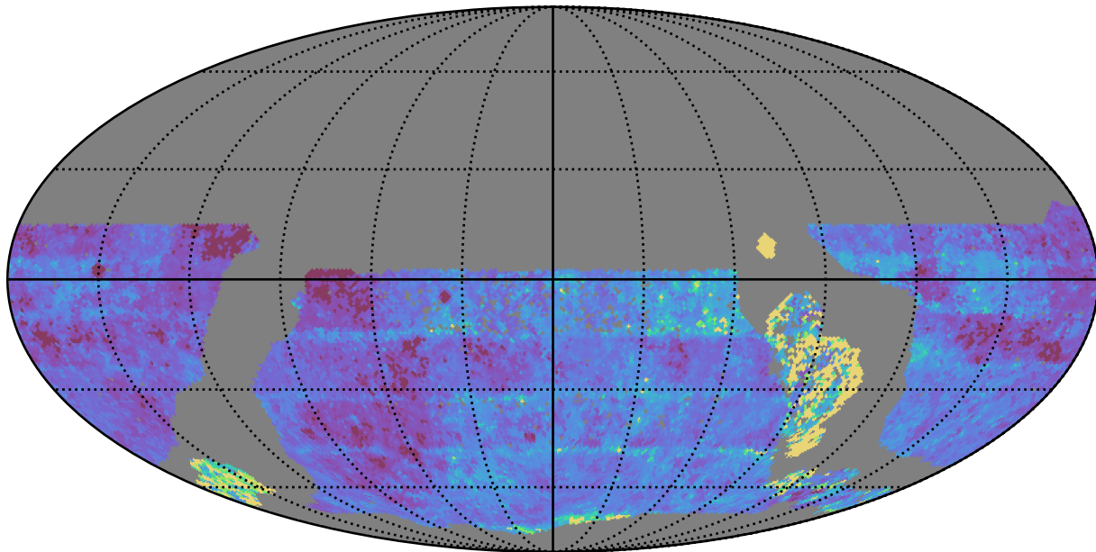
too_elab_r32_d3_giz_v3.4_10yrs WFD u band: Median Inter-Night Gap
