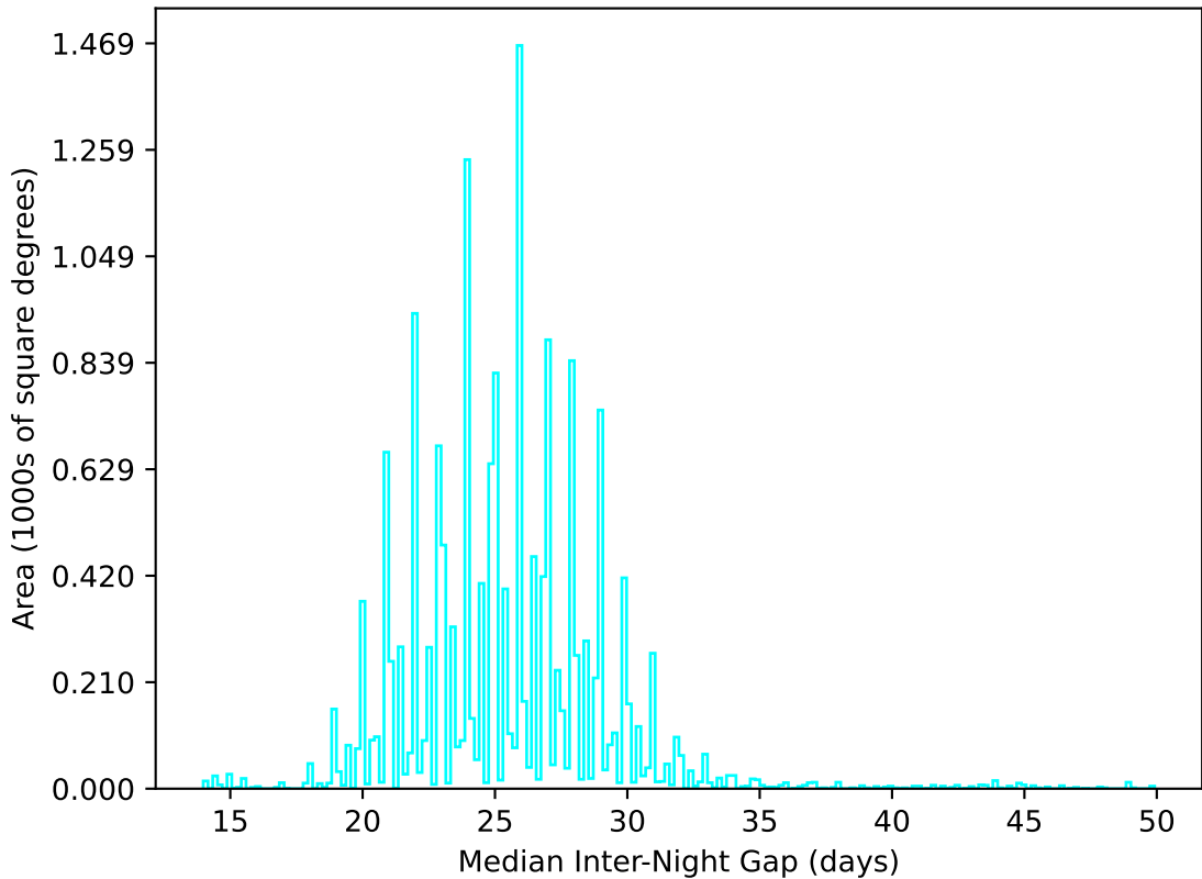
too_elab_r32_d3_giz_v3.4_10yrs WFD u band: Median Inter-Night Gap
