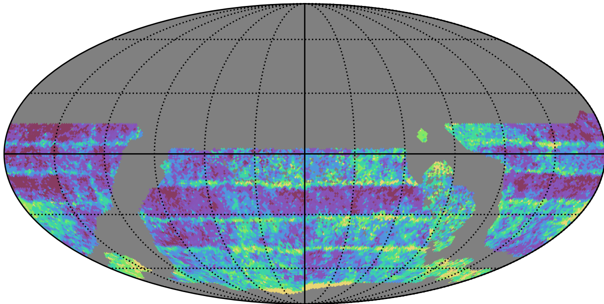
too_elab_r32_d3_giz_v3.4_10yrs WFD r band: Median Inter-Night Gap
