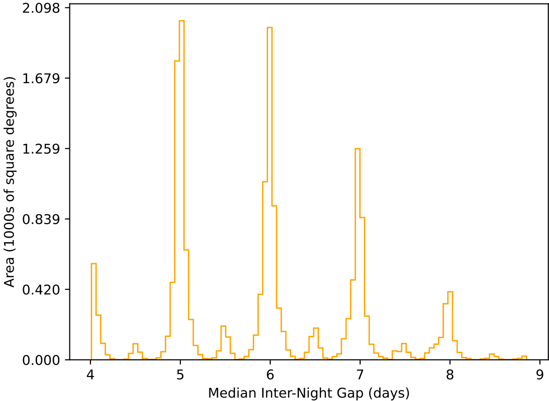
too_elab_r32_d3_giz_v3.4_10yrs WFD r band: Median Inter-Night Gap
