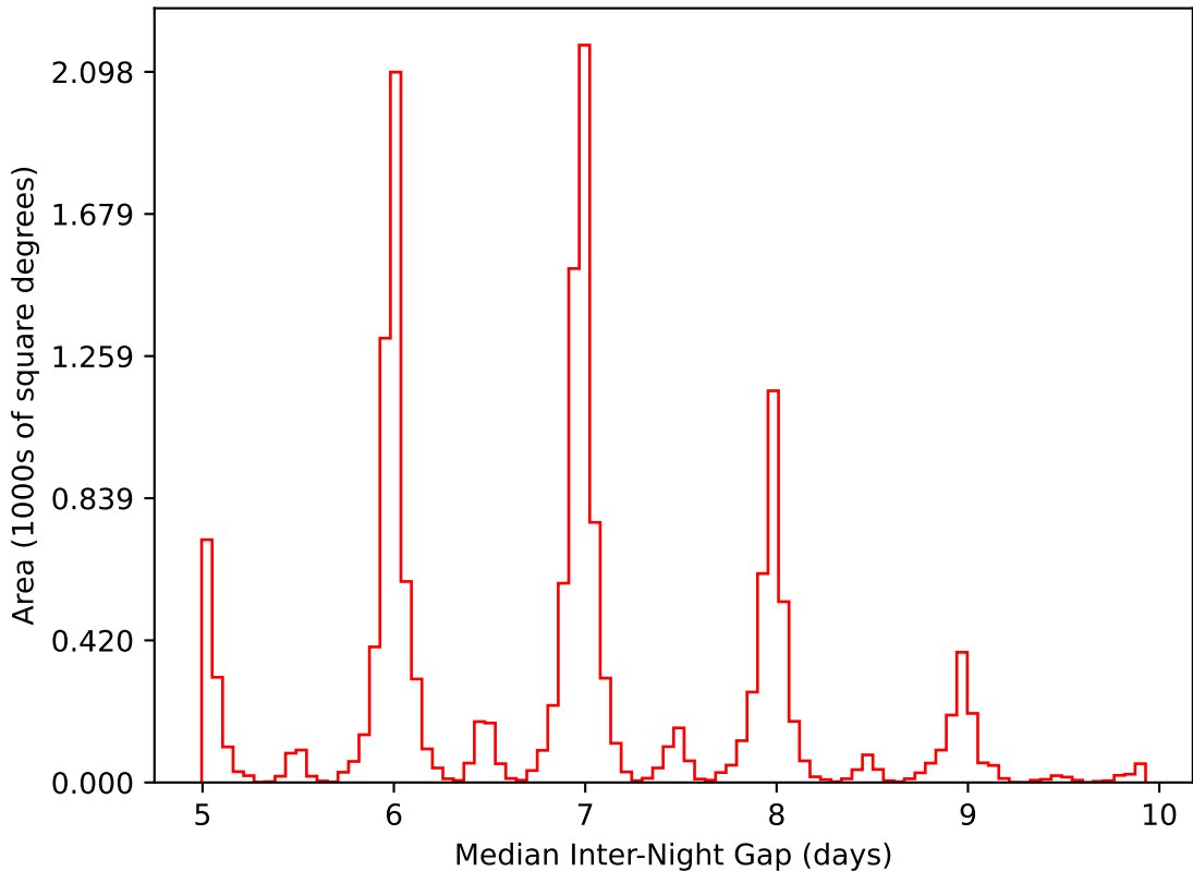
too_elab_r32_d3_giz_v3.4_10yrs WFD i band: Median Inter-Night Gap
