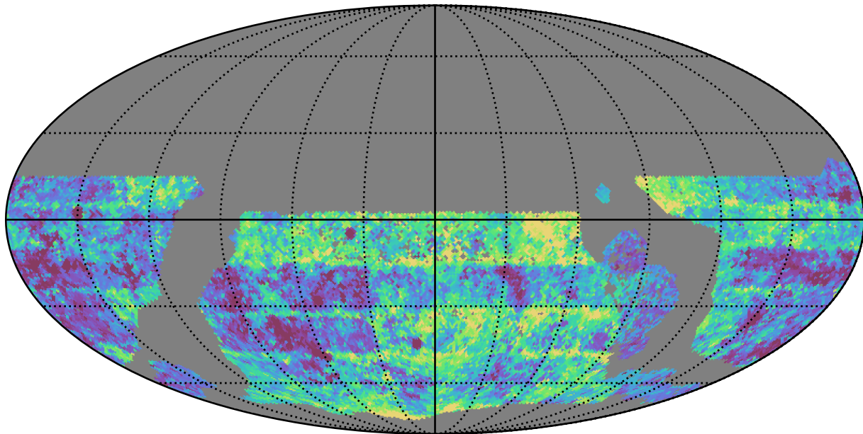
too_elab_r32_d3_giz_v3.4_10yrs WFD g band: Median Inter-Night Gap
