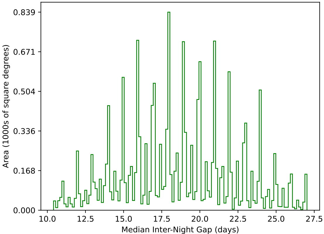
too_elab_r32_d3_giz_v3.4_10yrs WFD g band: Median Inter-Night Gap
