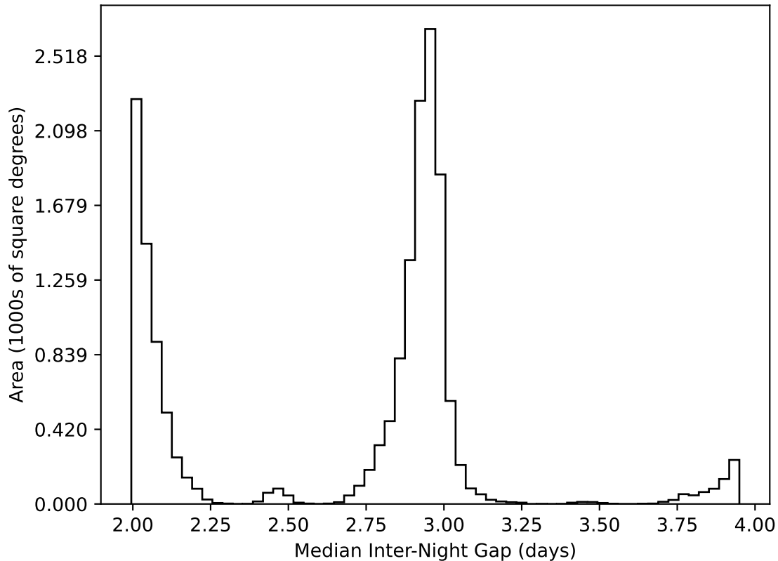
too_elab_r32_d3_giz_v3.4_10yrs WFD all bands: Median Inter-Night Gap
