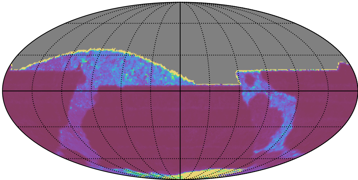
too_elab_r32_d3_giz_v3.4_10yrs All sky z band: Median Inter-Night Gap
