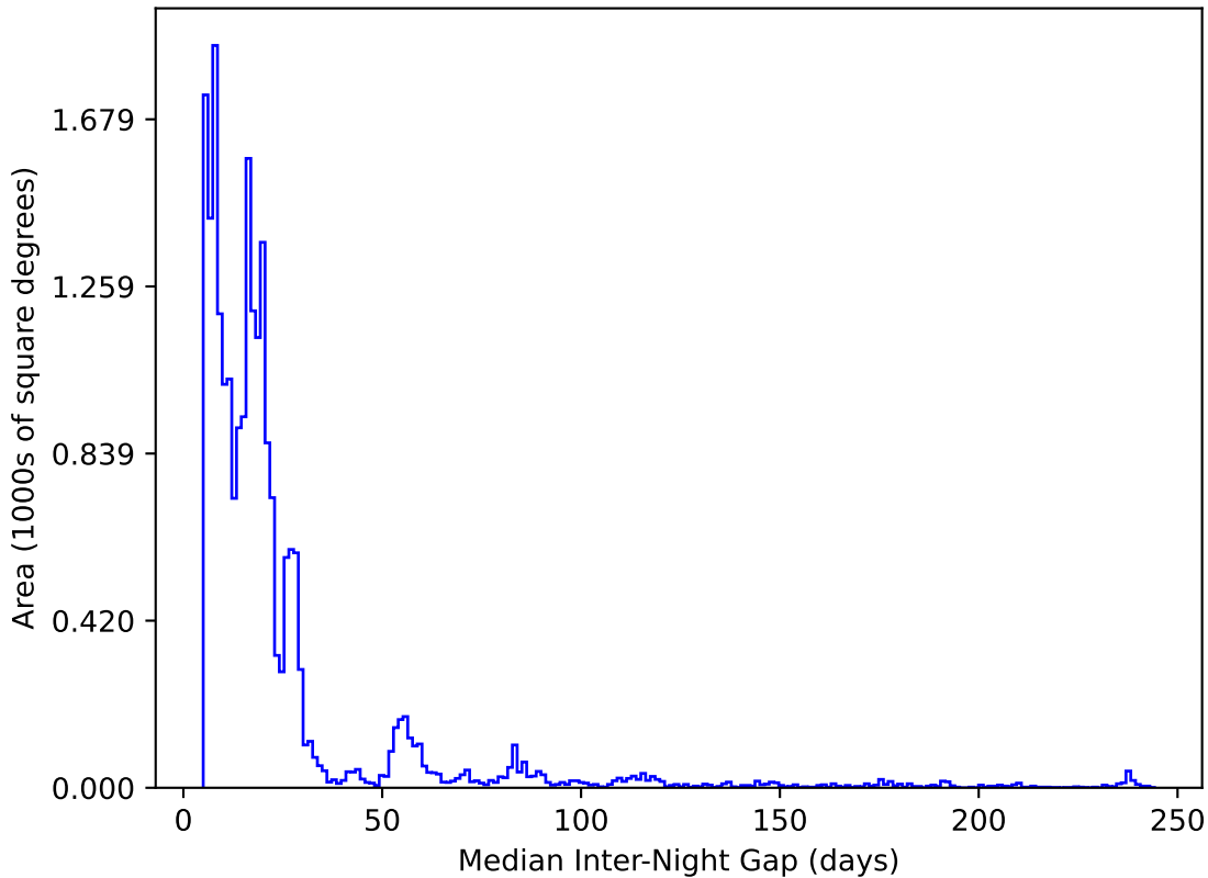
too_elab_r32_d3_giz_v3.4_10yrs All sky y band: Median Inter-Night Gap
