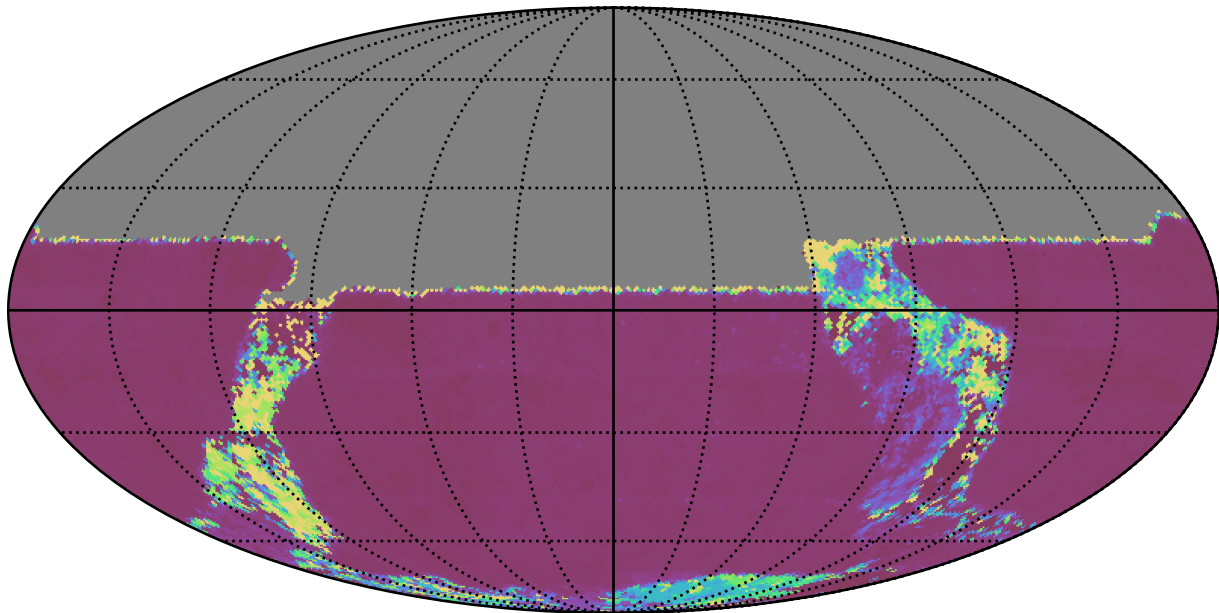
too_elab_r32_d3_giz_v3.4_10yrs All sky u band: Median Inter-Night Gap
