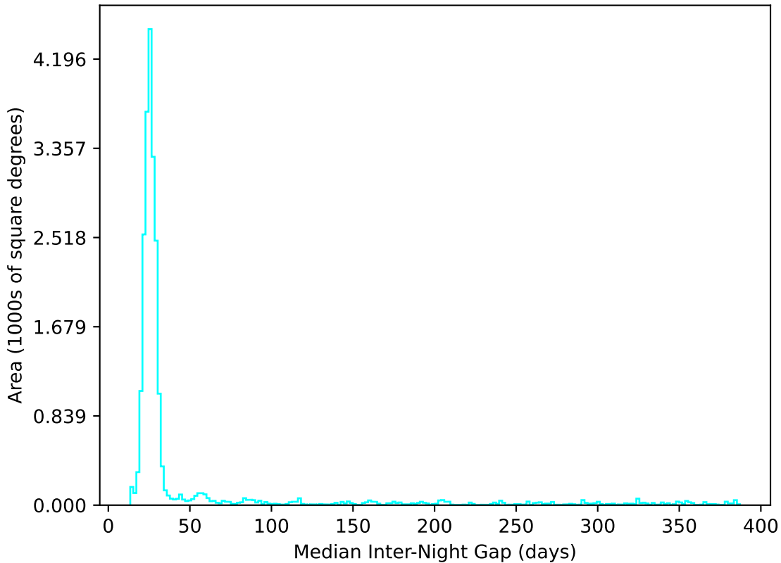
too_elab_r32_d3_giz_v3.4_10yrs All sky u band: Median Inter-Night Gap
