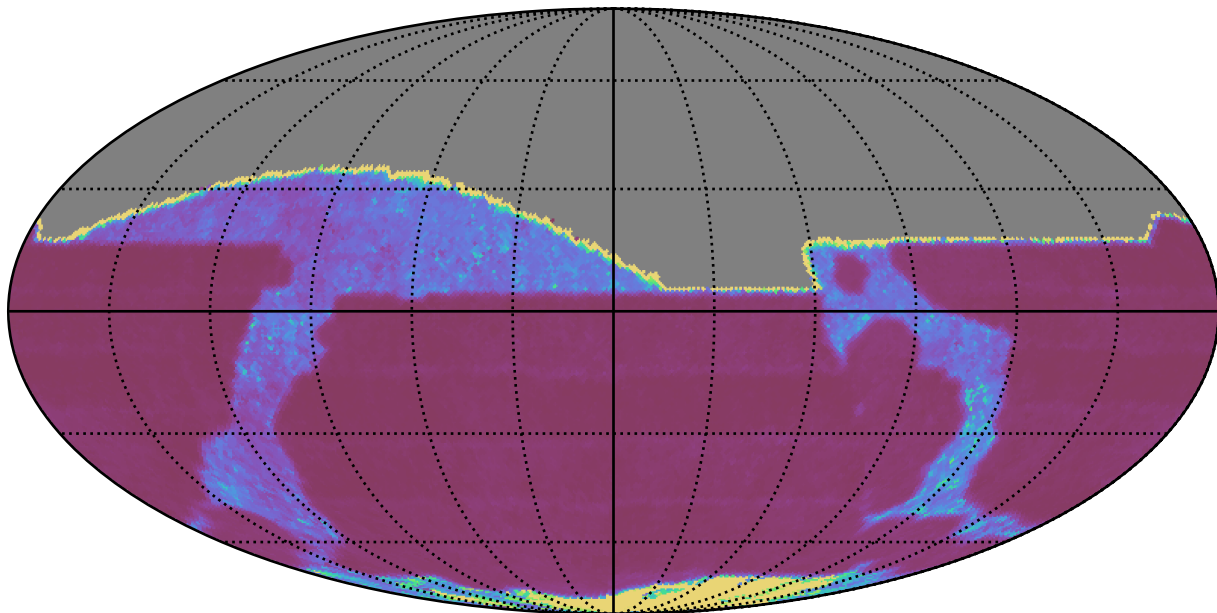
too_elab_r32_d3_giz_v3.4_10yrs All sky r band: Median Inter-Night Gap
