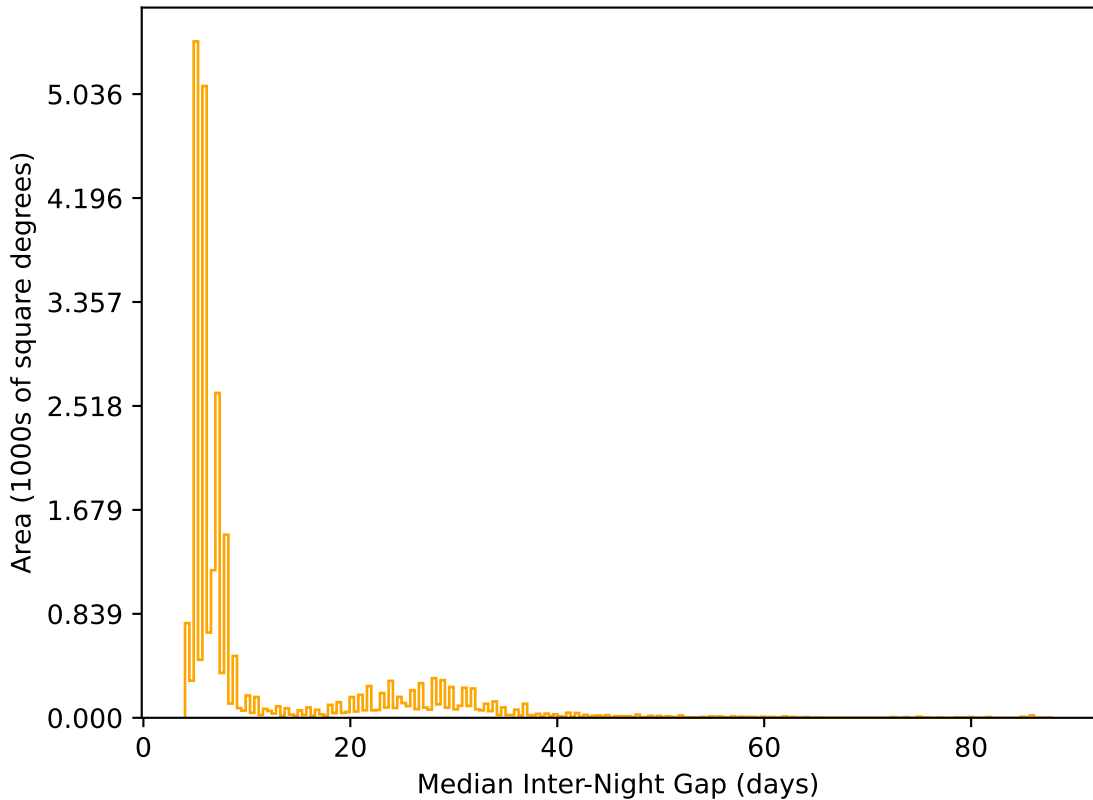
too_elab_r32_d3_giz_v3.4_10yrs All sky r band: Median Inter-Night Gap
