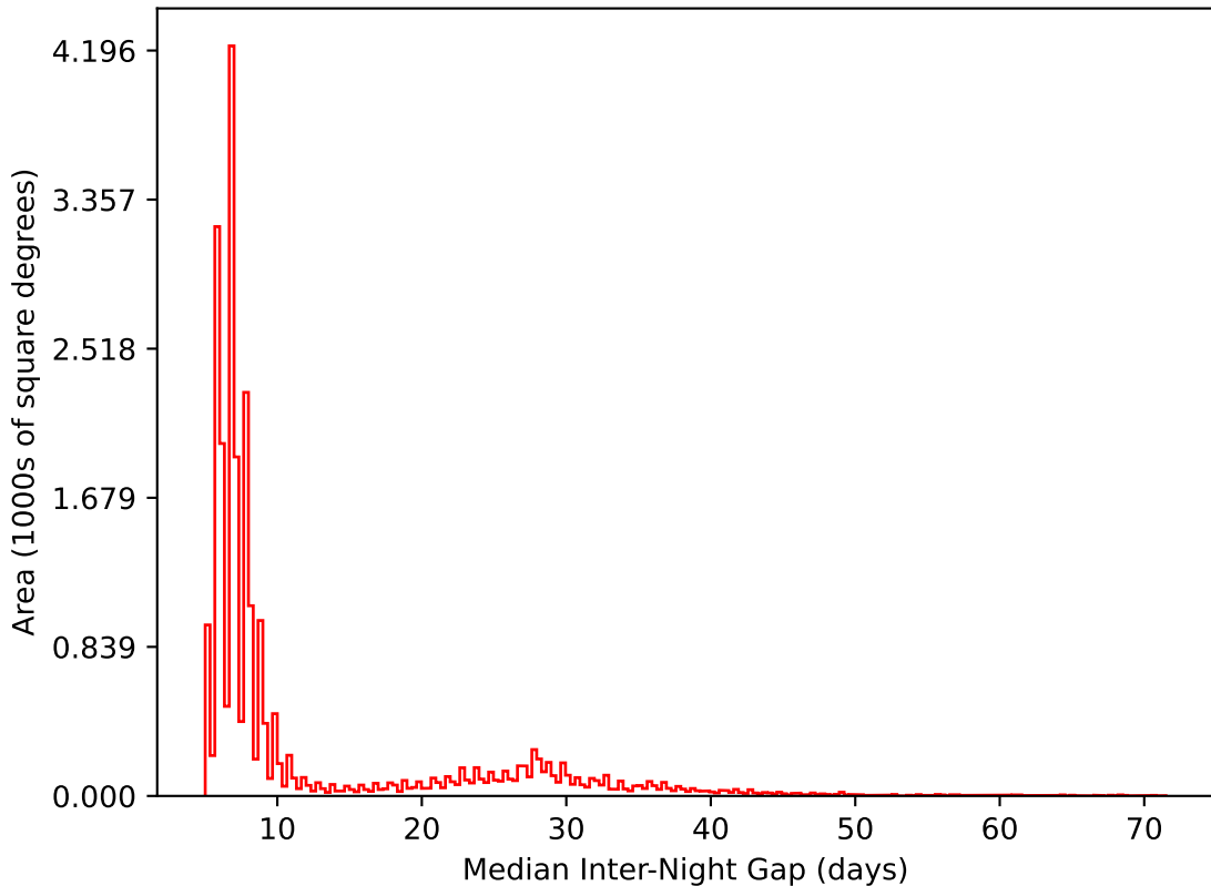
too_elab_r32_d3_giz_v3.4_10yrs All sky i band: Median Inter-Night Gap
