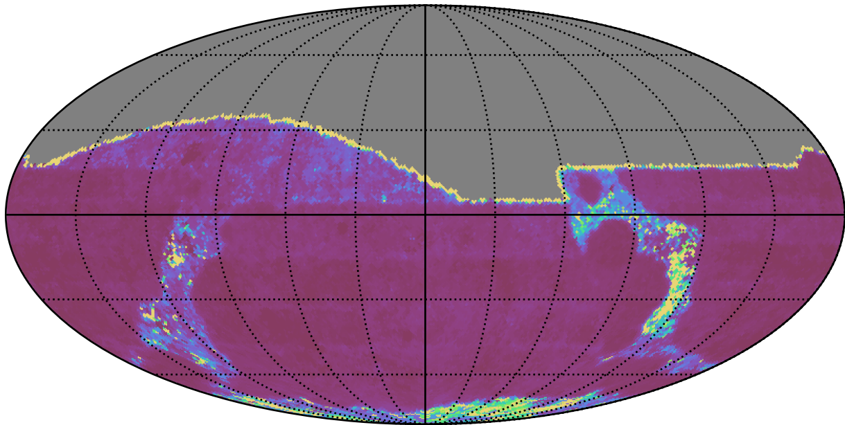
too_elab_r32_d3_giz_v3.4_10yrs All sky g band: Median Inter-Night Gap
