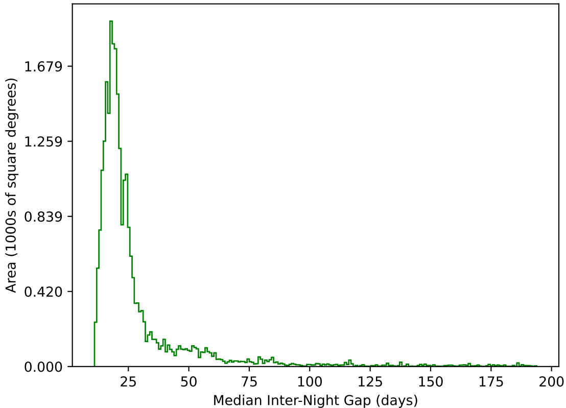
too_elab_r32_d3_giz_v3.4_10yrs All sky g band: Median Inter-Night Gap
