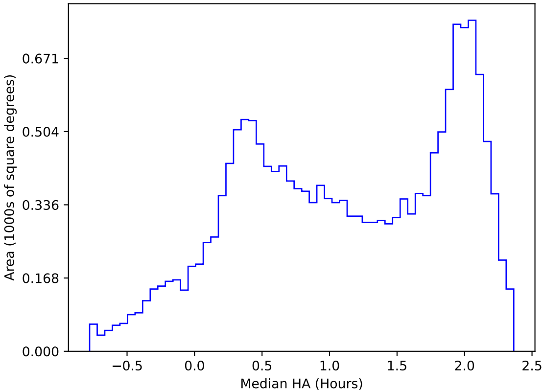
too_elab_r32_d3_giz_v3.4_10yrs WFD z band: Median HA
