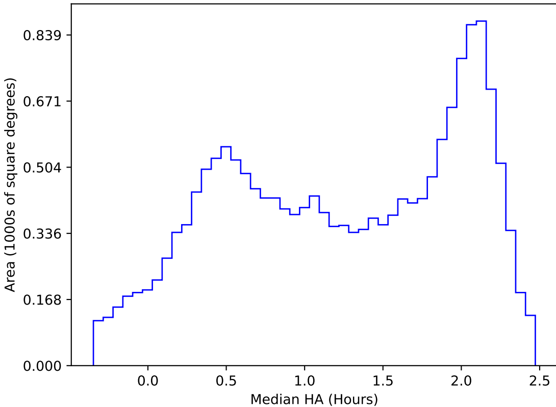
too_elab_r32_d3_giz_v3.4_10yrs WFD y band: Median HA
