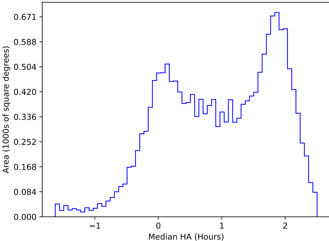
too_elab_r32_d3_giz_v3.4_10yrs WFD u band: Median HA
