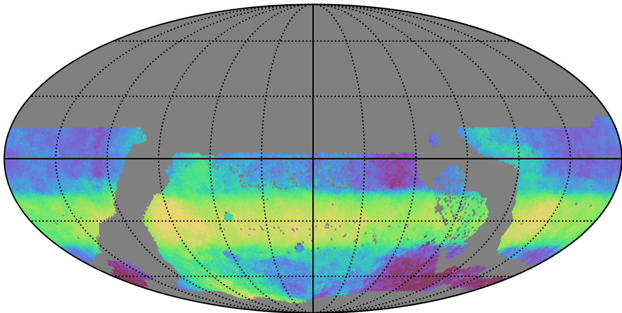
too_elab_r32_d3_giz_v3.4_10yrs WFD r band: Median HA
