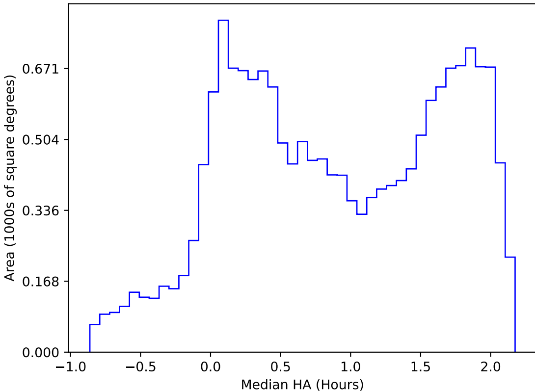
too_elab_r32_d3_giz_v3.4_10yrs WFD r band: Median HA
