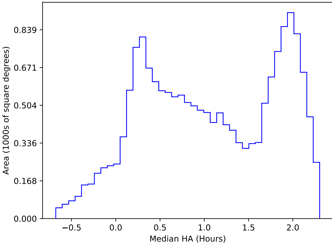
too_elab_r32_d3_giz_v3.4_10yrs WFD i band: Median HA
