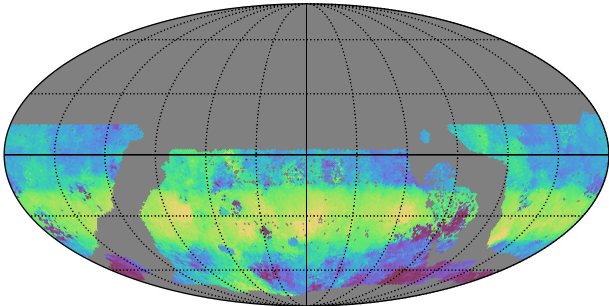
too_elab_r32_d3_giz_v3.4_10yrs WFD g band: Median HA
