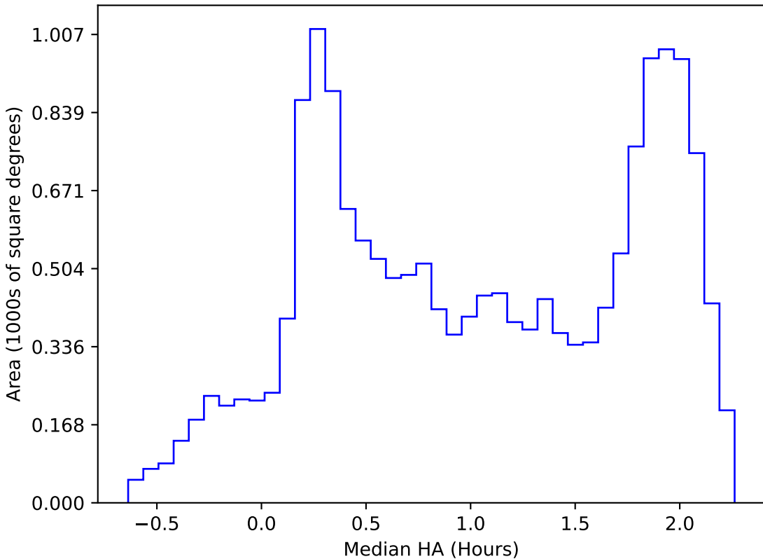
too_elab_r32_d3_giz_v3.4_10yrs WFD all bands: Median HA
