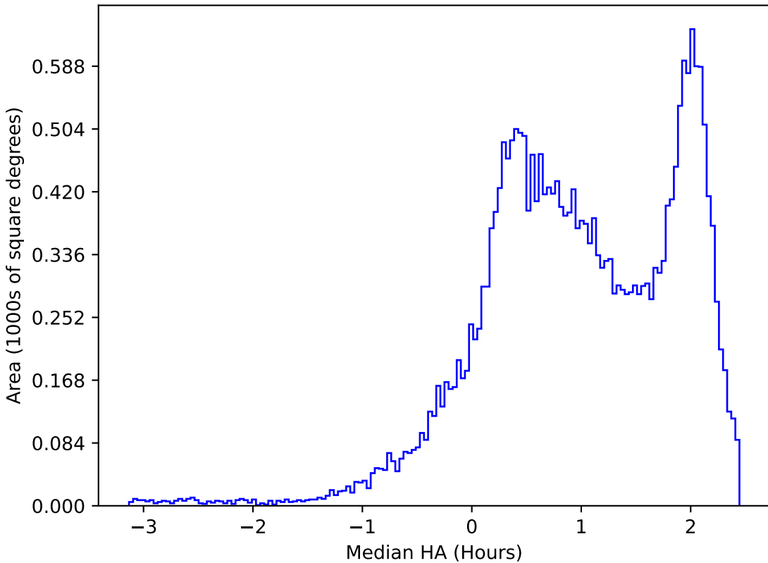
too_elab_r32_d3_giz_v3.4_10yrs All sky z band: Median HA
