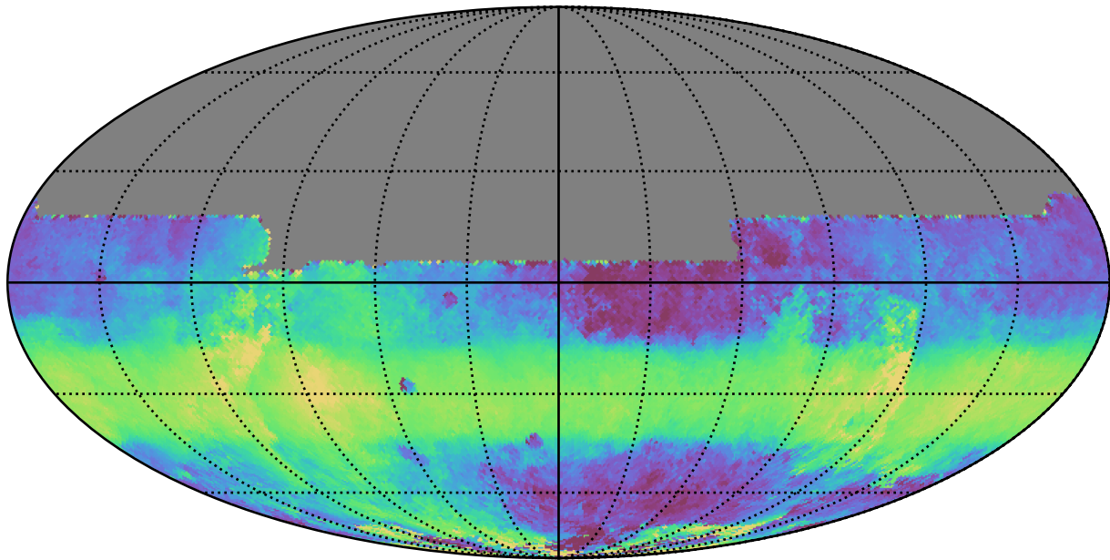
too_elab_r32_d3_giz_v3.4_10yrs All sky y band: Median HA
