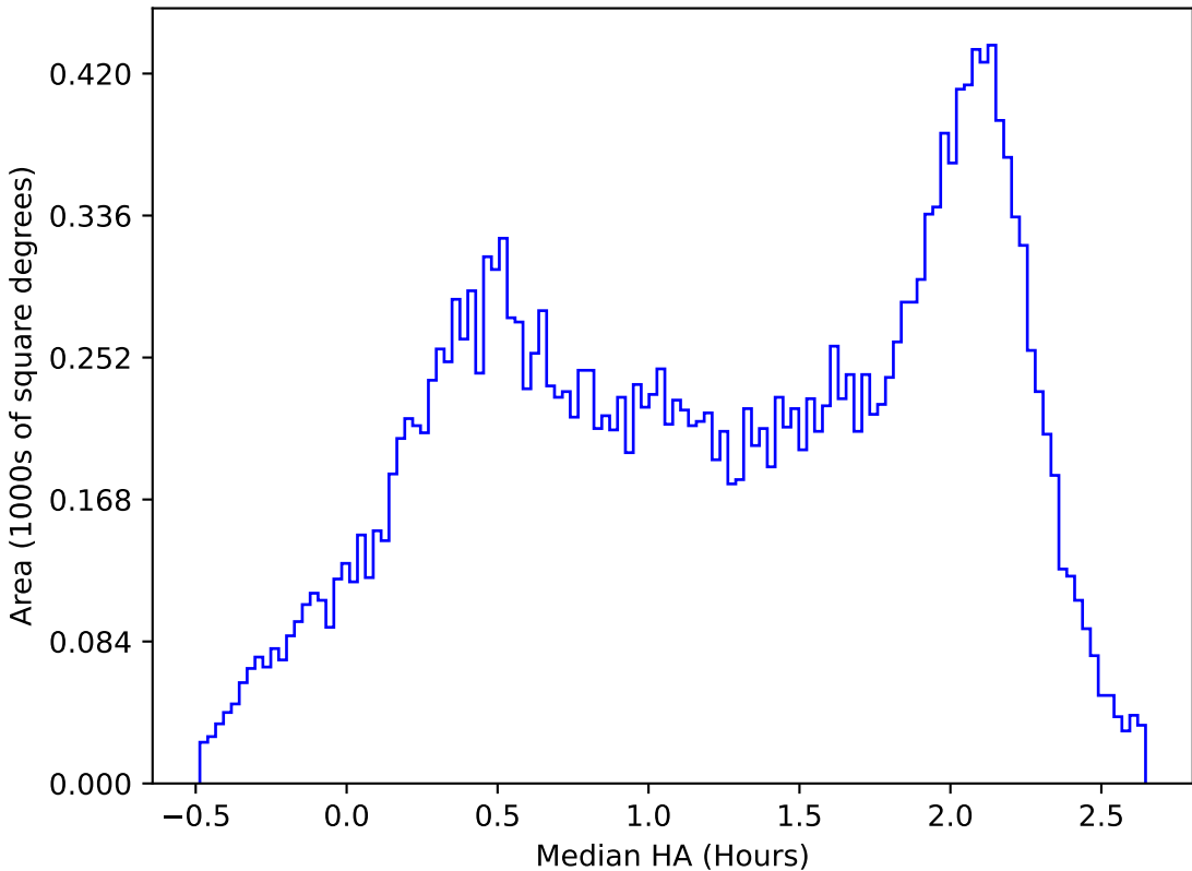
too_elab_r32_d3_giz_v3.4_10yrs All sky y band: Median HA
