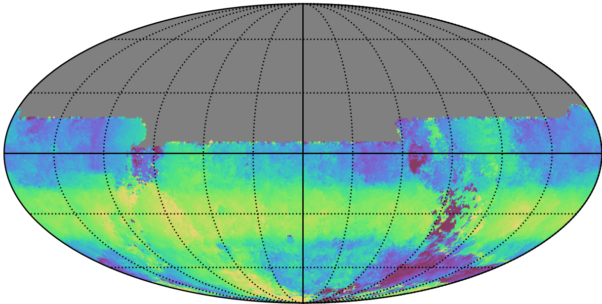
too_elab_r32_d3_giz_v3.4_10yrs All sky u band: Median HA
