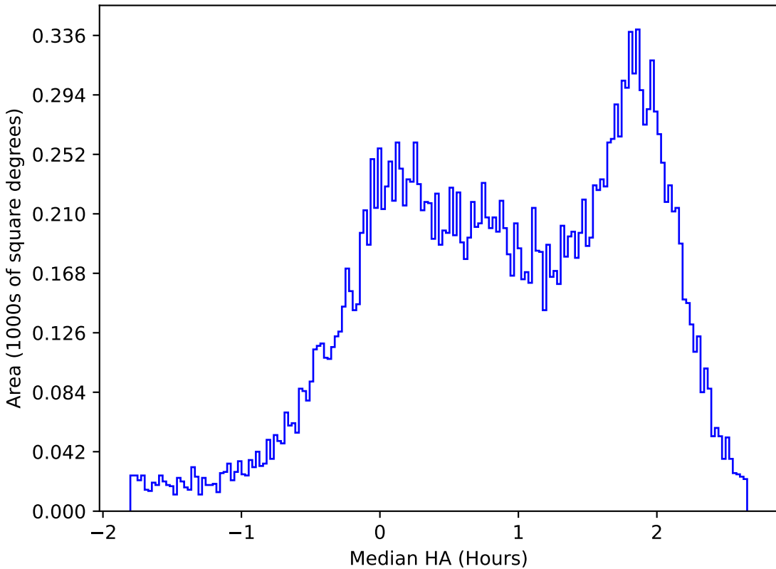
too_elab_r32_d3_giz_v3.4_10yrs All sky u band: Median HA
