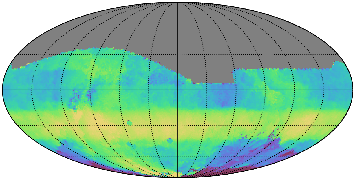
too_elab_r32_d3_giz_v3.4_10yrs All sky r band: Median HA
