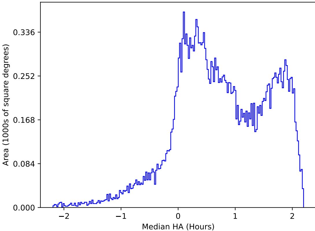
too_elab_r32_d3_giz_v3.4_10yrs All sky r band: Median HA
