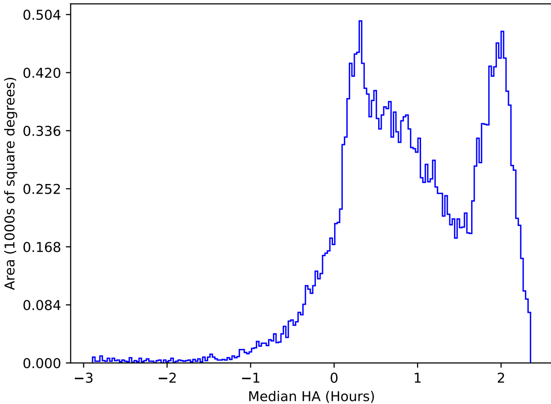
too_elab_r32_d3_giz_v3.4_10yrs All sky i band: Median HA
