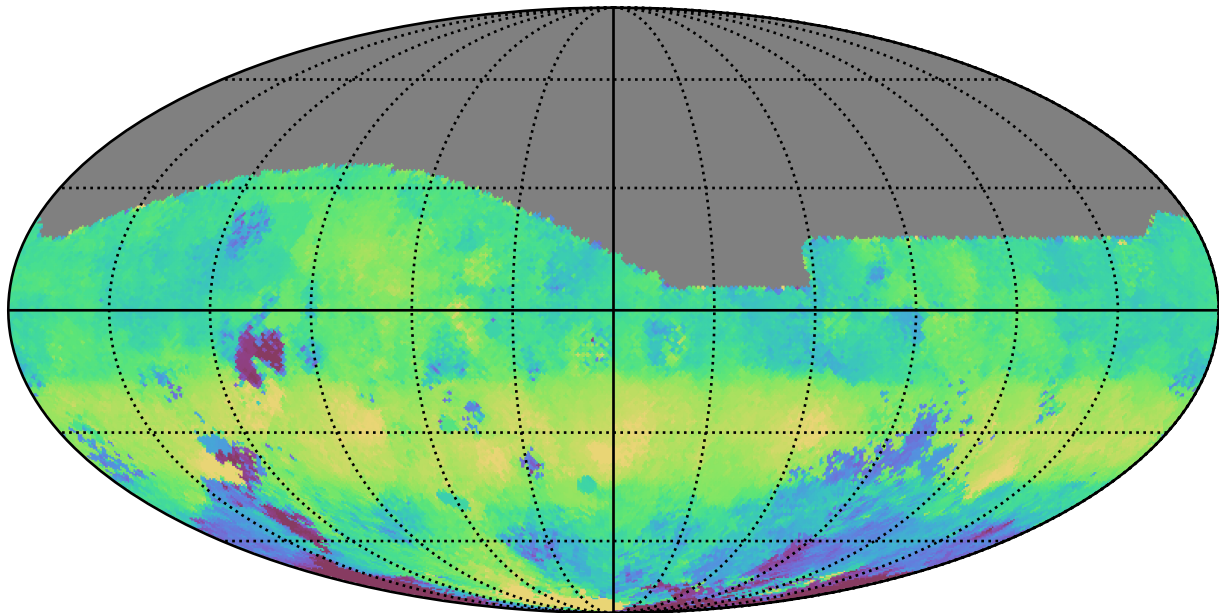
too_elab_r32_d3_giz_v3.4_10yrs All sky g band: Median HA
