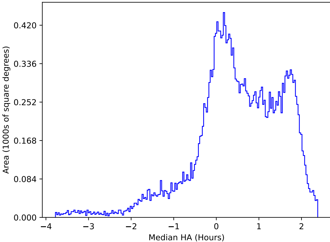
too_elab_r32_d3_giz_v3.4_10yrs All sky g band: Median HA
