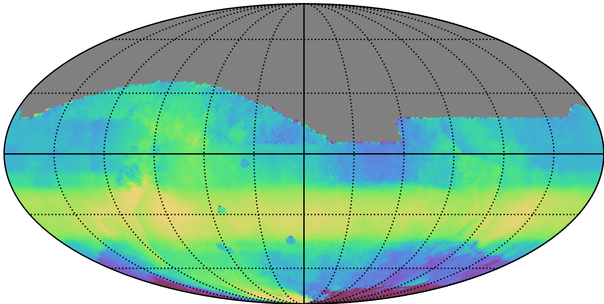
too_elab_r32_d3_giz_v3.4_10yrs All sky all bands: Median HA
