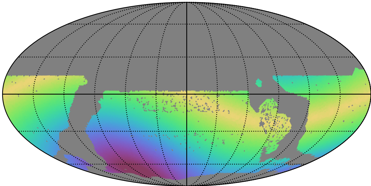
too_elab_r32_d3_giz_v3.4_10yrs WFD z band: Max solarElong
