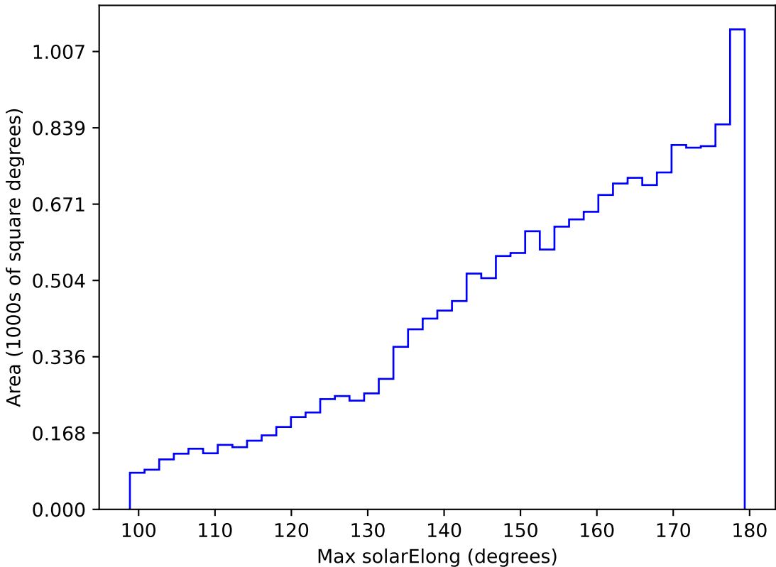
too_elab_r32_d3_giz_v3.4_10yrs WFD z band: Max solarElong
