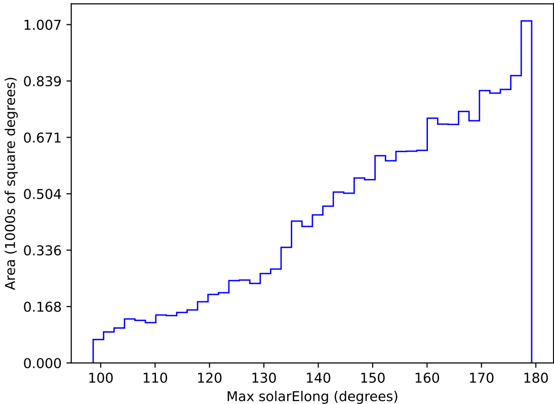
too_elab_r32_d3_giz_v3.4_10yrs WFD y band: Max solarElong
